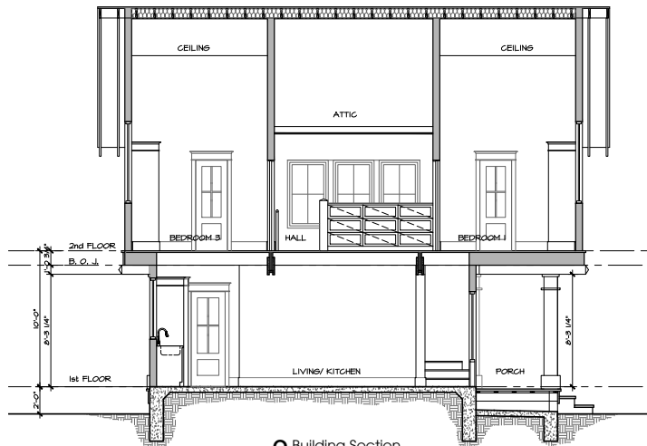
3 Building Section SCALE: 1/4" = 1'-0"
